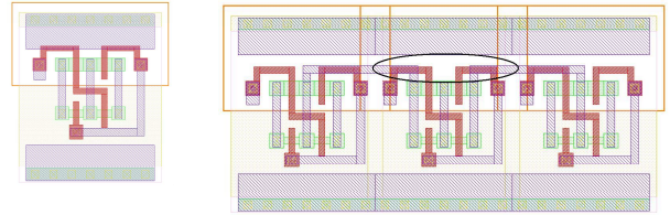
Figure 2. The layout of a 2:1 mux and a 3-input Lookup Table with the additional area highlighted.
