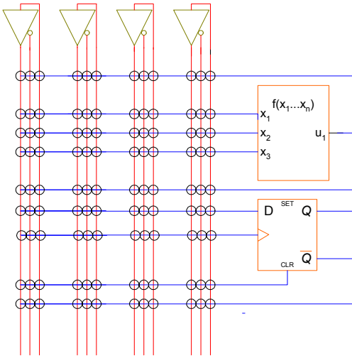
Figure 3. Depiction of the CLB showing local connectivity.
